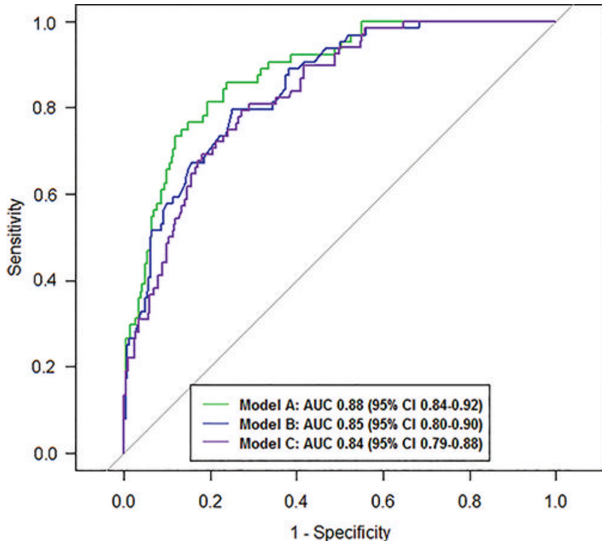
Figure 3. Graph shows areas under the receiver operating characteristic curves (AUCs) of three prediction models for true-positive MRI screening. Model A (green): The full model, including all clinical characteristics and MRI findings based on 328 participants. Model B (blue): The reduced model, including the variables age, menopausal status, number of first-degree relatives with breast cancer, history of breast biopsy, MRI Breast Imaging Reporting and Data System classification, and initial phase kinetics. Model C (purple): The model based on readily available data, including all MRI findings based on 369 participants.
