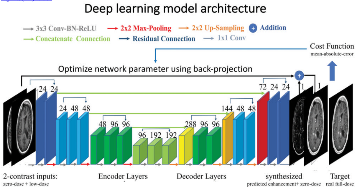
Figure 3. Visualization of the deep learning model architecture that was used.
