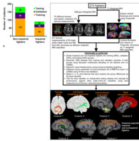
Figure 2. (a) Bar graph shows total impaired and nonimpaired fighters who were included for classification. Subjects in each fighter population were divided into training (60 percent; 110 of 182 nonimpaired and 55 of 91 impaired fighters), validation (20 percent; 36 of 182 nonimpaired and 18 of 91 impaired fighters), and testing (20 percent; 36 of 182 nonimpaired and 18 of 91 impaired fighters) sets. Training and validation sample set were shuffled 10 times to estimate best training parameters. Numbers represent actual number of subjects in each set. (b) Pipeline used to generate features from diffusion-weighted and T1-weighted MR imaging is shown. Brief description of classifier for which least absolute shrinkage and selection operator ( LASSO ) and radial basis functional networks ( RBFNs ) were used, and imaging features associated with cognition in our cohort of active professional fighters, overlaid on Montreal Neurological Institute 152 template, is also shown. AAL = anatomical atlas labeling, MD = mean diffusivity, DTI = diffusion-tensor imaging.
