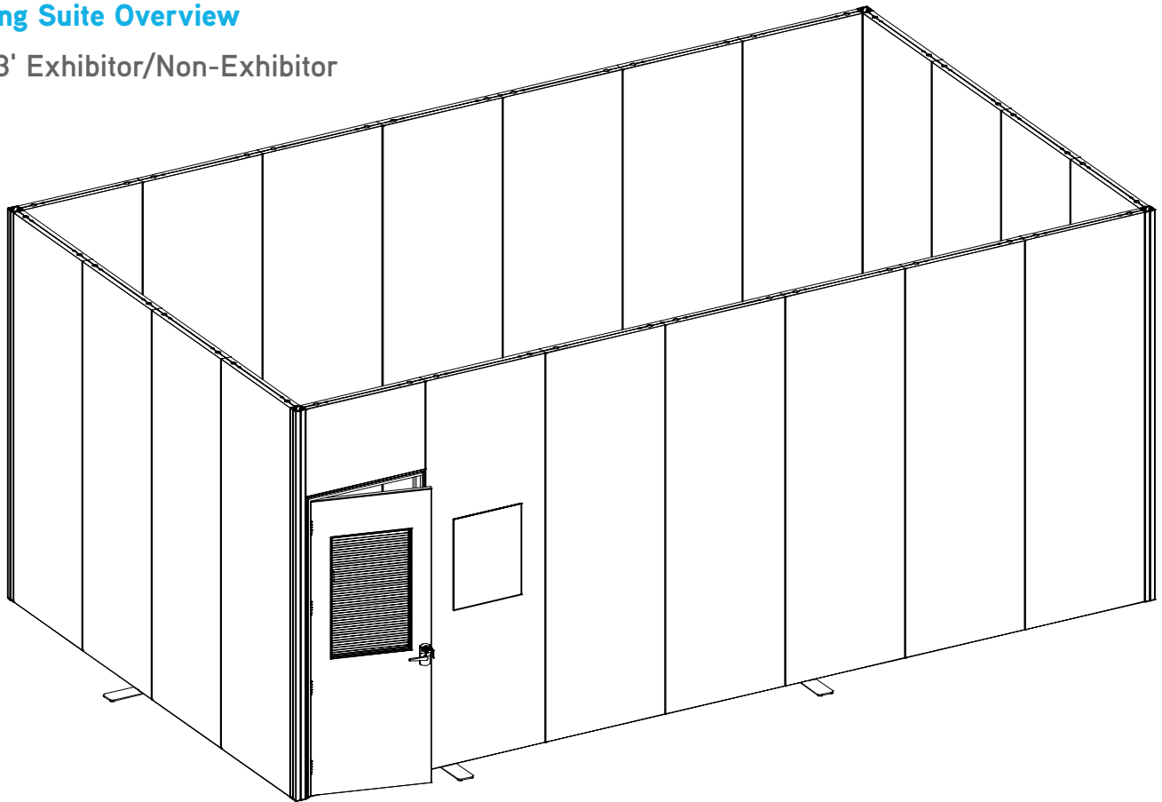
ISO VIEW
